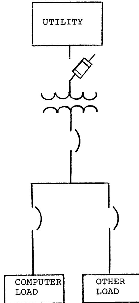
FIG. 1B NON-DEDICATED LINE
