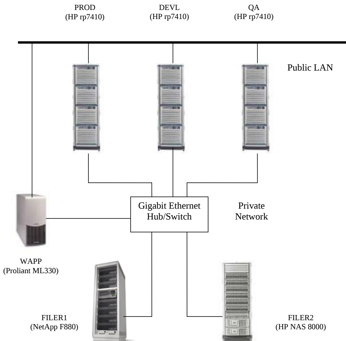
Figure 2 NAS-based Landscape
